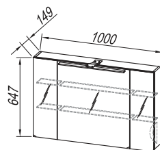
TOO 100 -LED, SW, S
