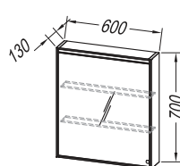
TO 60 BL - LED, SW, S
