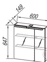
TOO 60 -LED, SW, S
